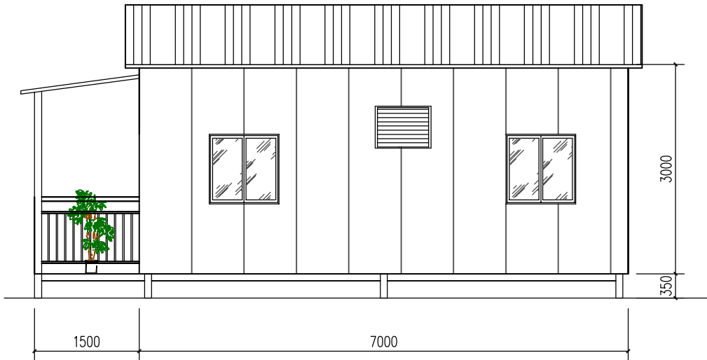
Back Elevation
