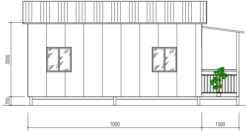
Front Elevation
