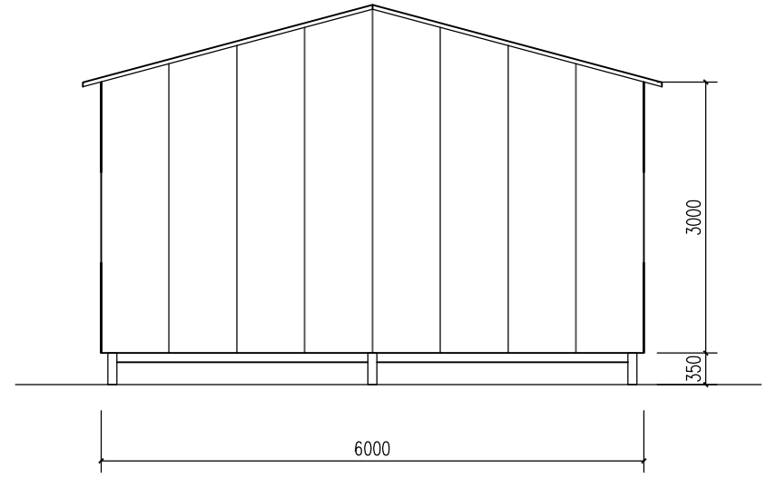
Left Elevation
